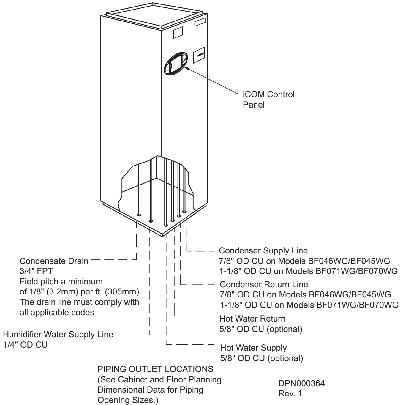
Figure 8 Piping connections for water/glycol and GLYCOOL units - Downflow models
