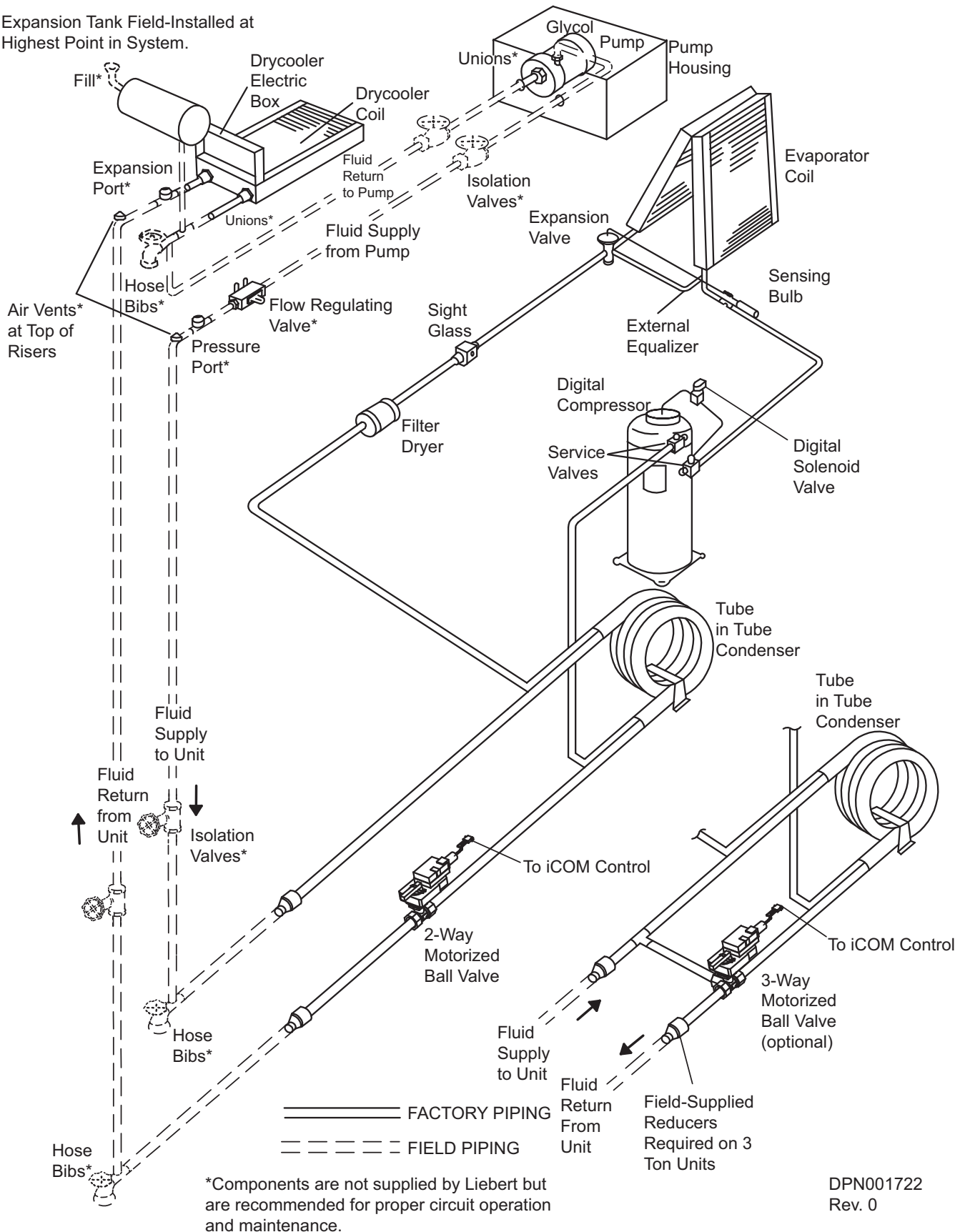
Figure 26 General arrangement—Glycol-cooled models with digital scroll
