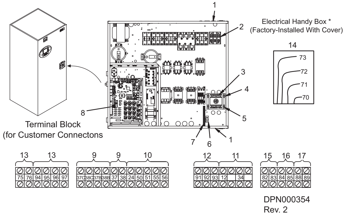
Figure 12 Electrical connections
