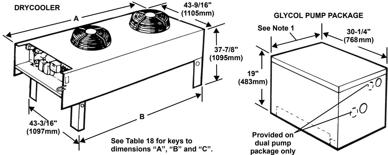
Figure 23 Drycoolers and pump packages
