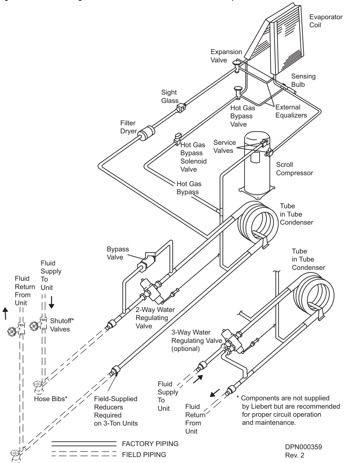
Figure 19 General arrangement—Water-cooled models with scroll compressor
