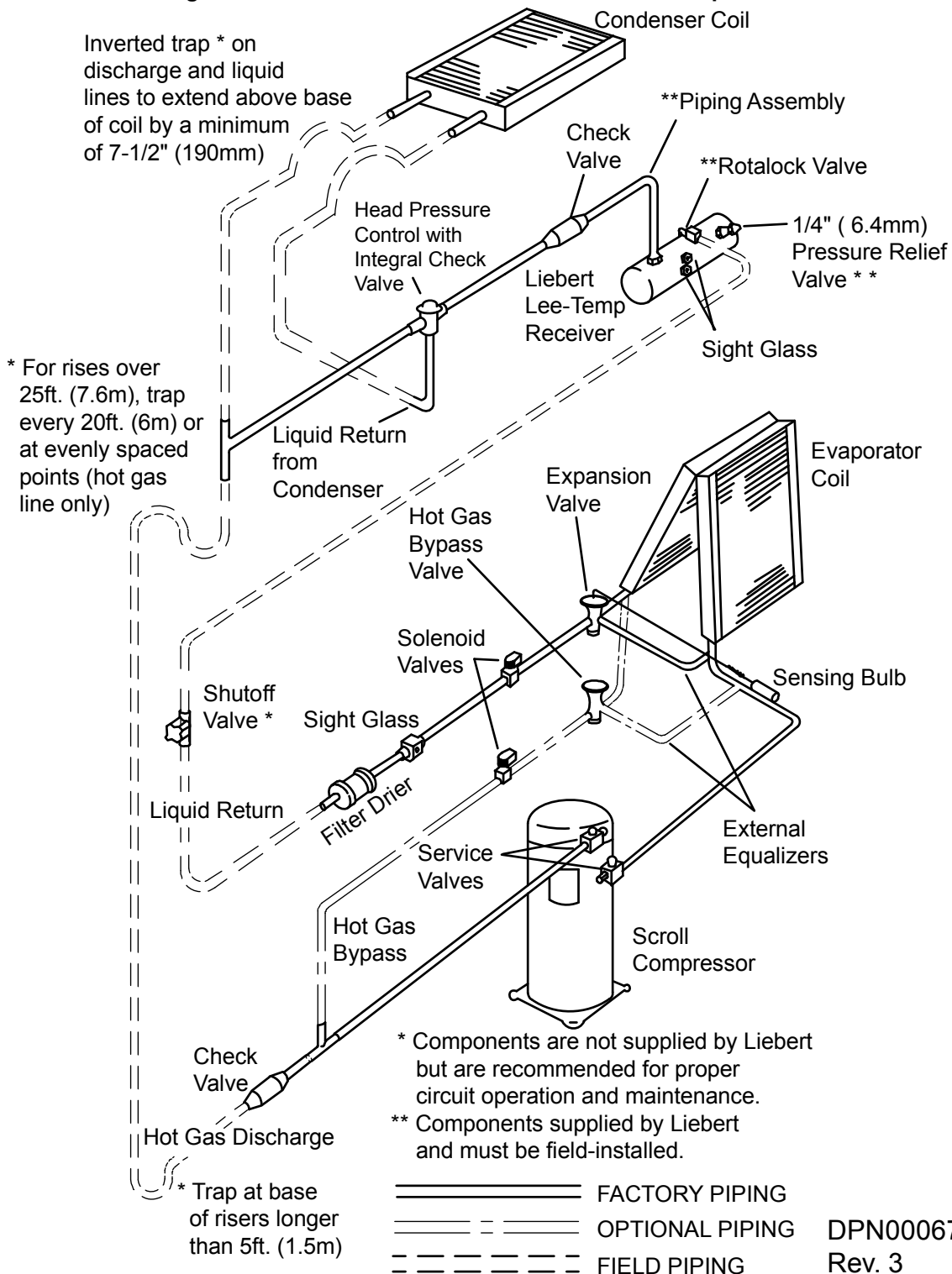
Figure 17 General arrangement—Air-cooled models with Liebert Lee-Temp™
