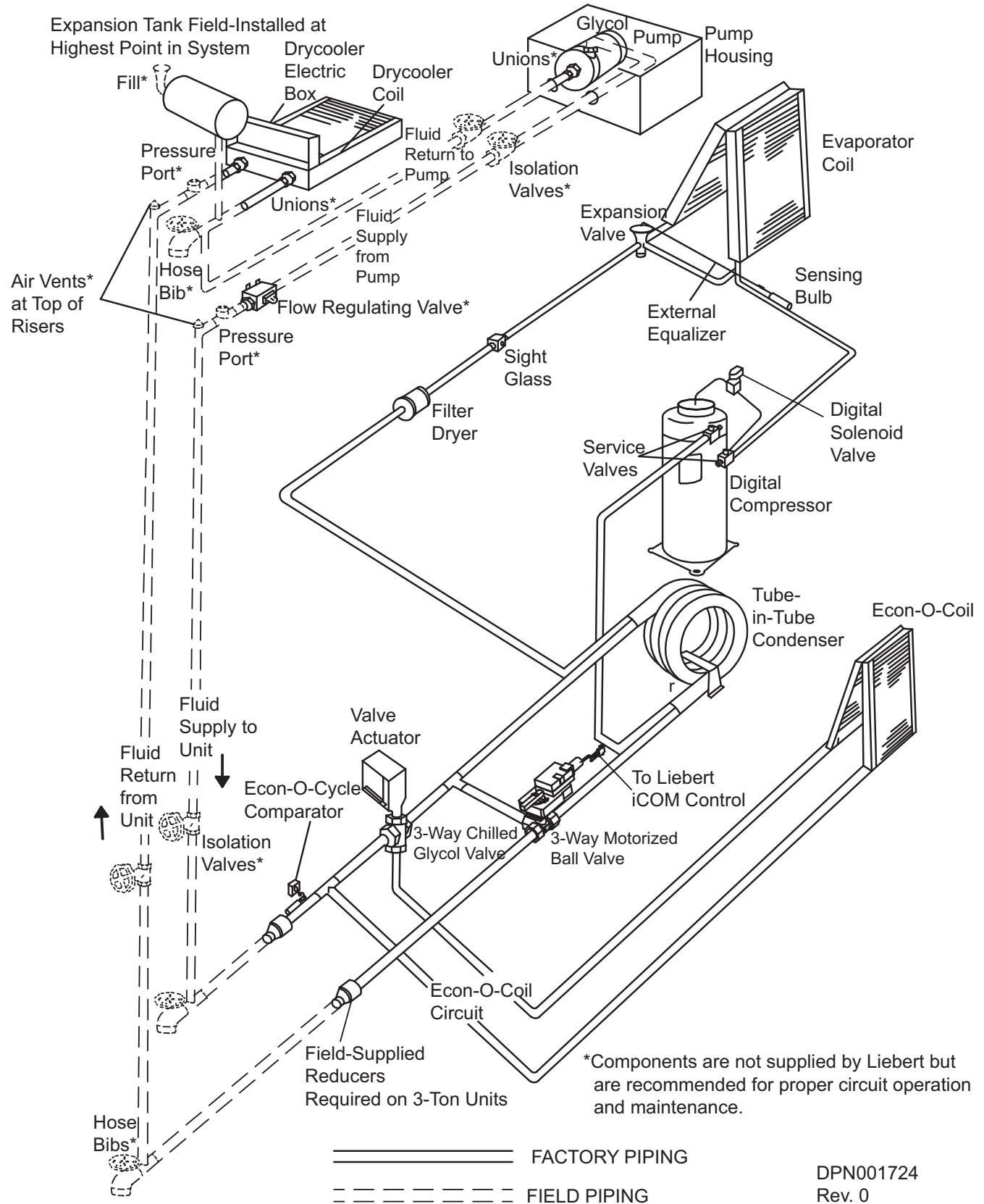
Figure 28 General arrangement—GLYCOOL models with digital scroll compressor
