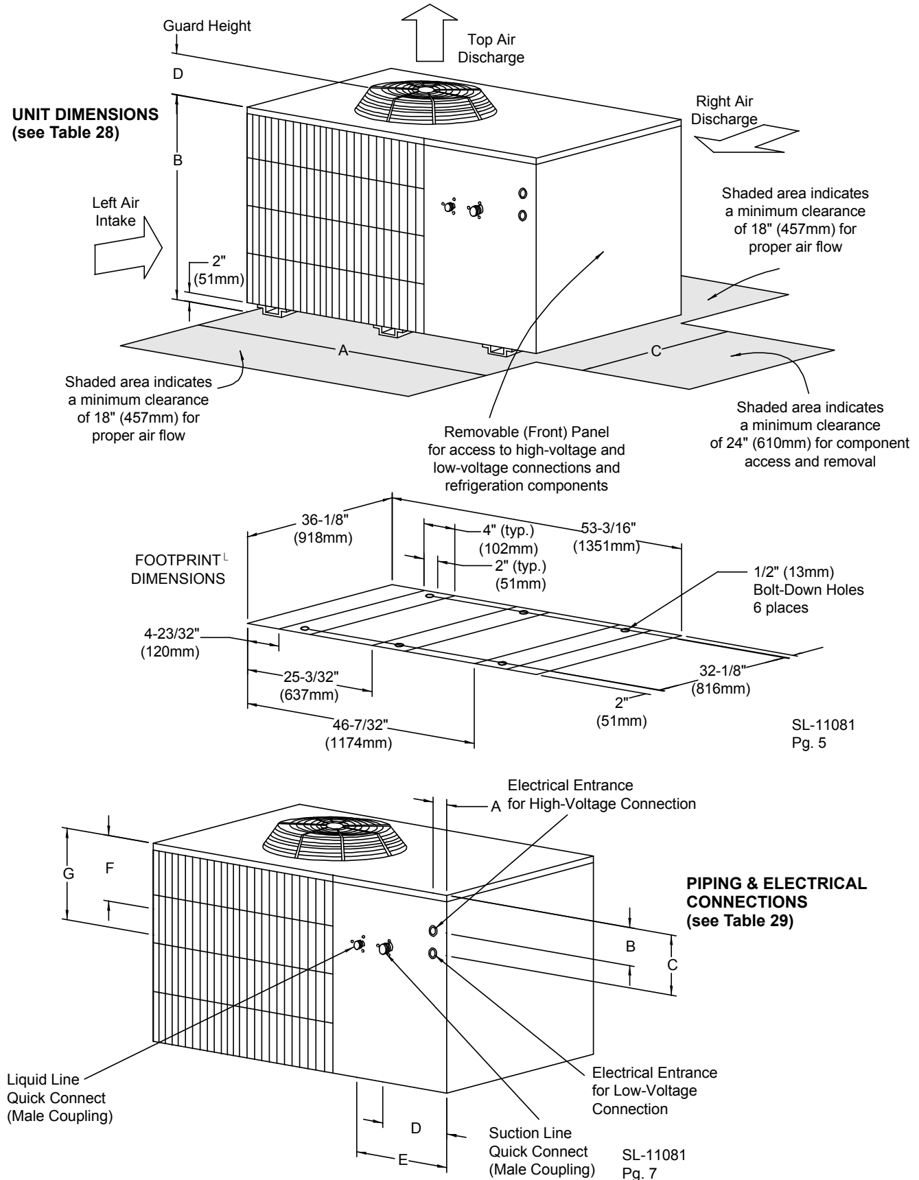
Figure 33 Outdoor air-cooled condensing unit—top air discharge models
