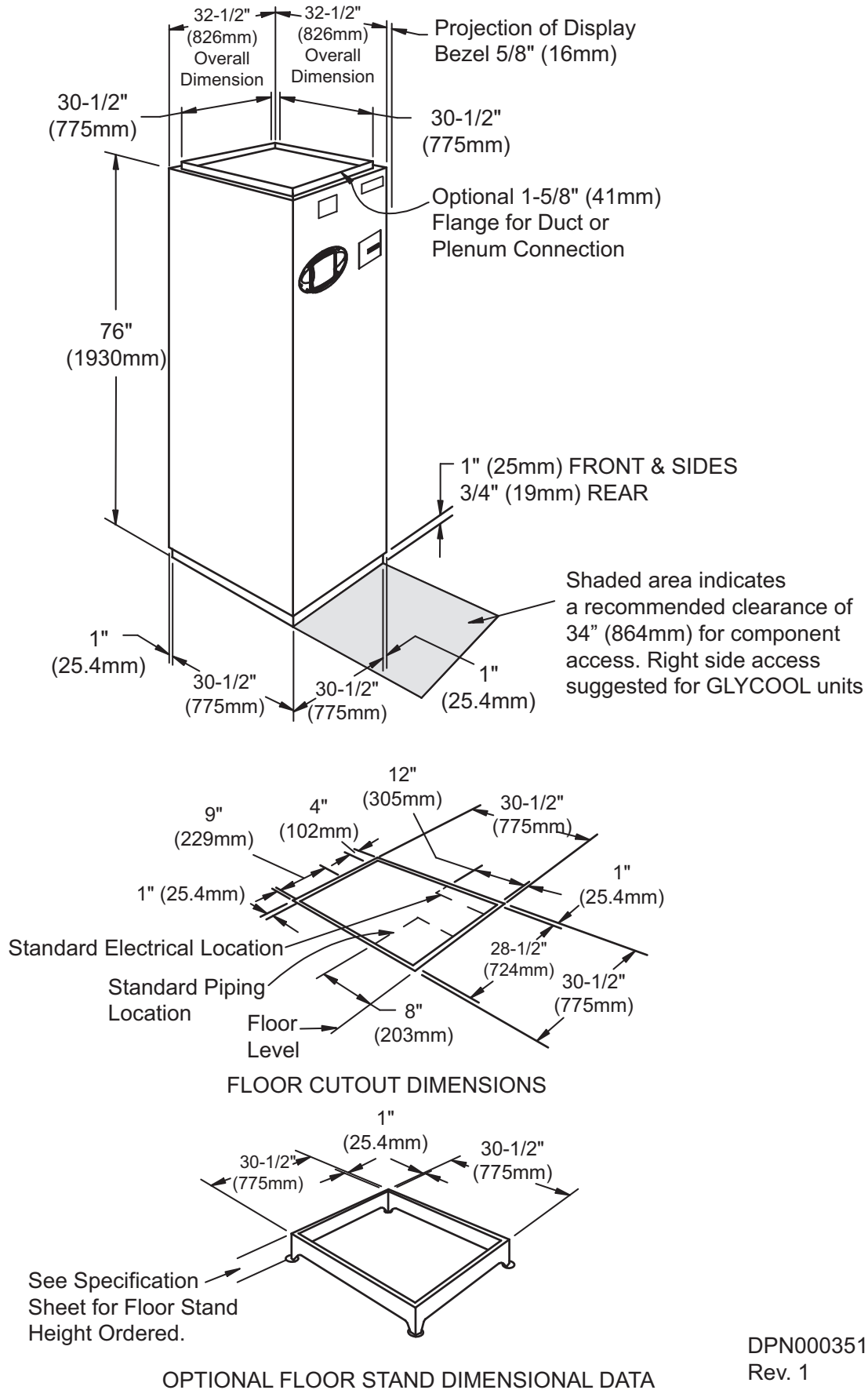
Figure 3 Downflow (BF) cabinet dimensions
