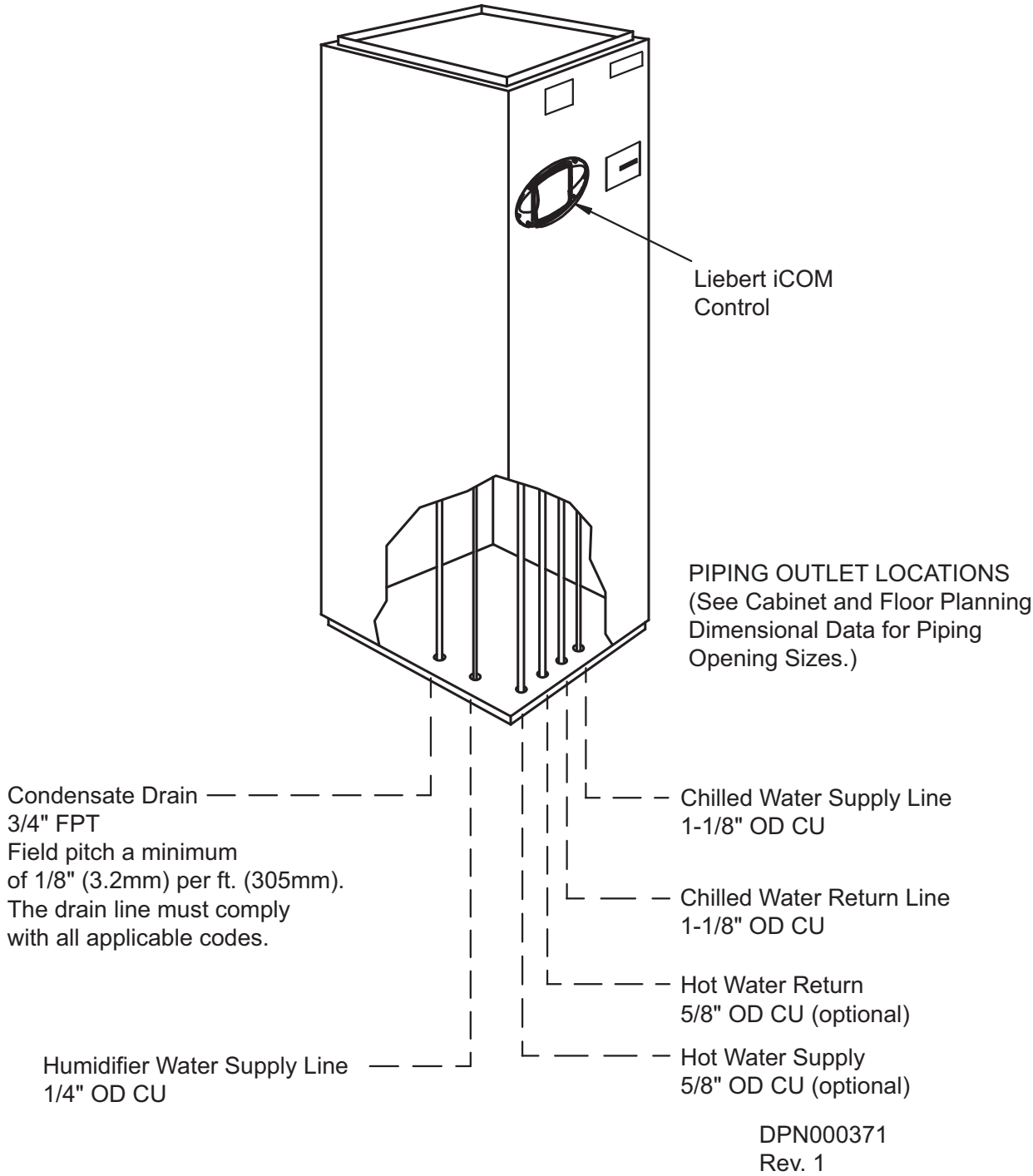
Figure 10 Piping connections for chilled water self-contained units - Downflow models
