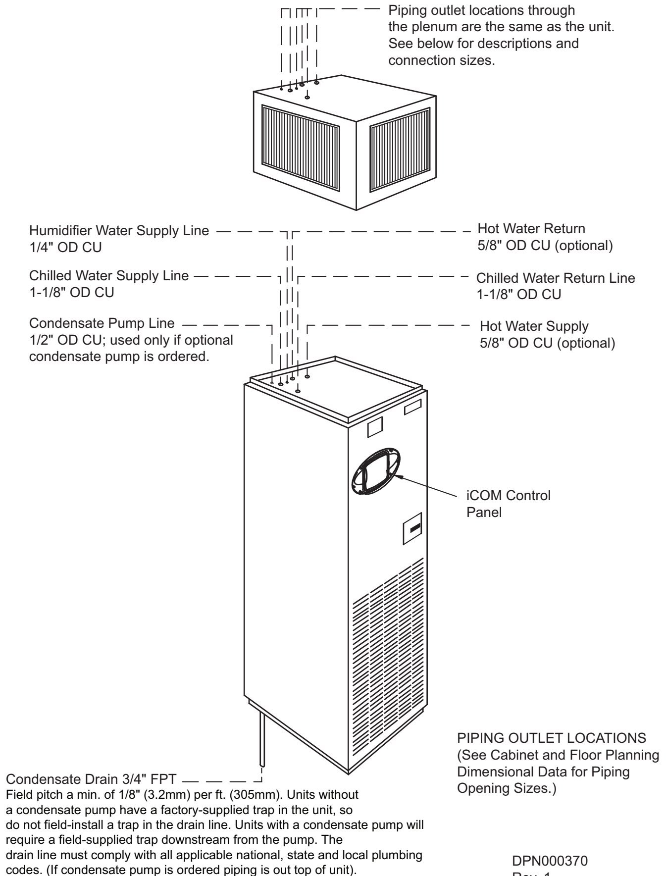
Figure 11 Piping connections for chilled water self-contained units - Upflow models
