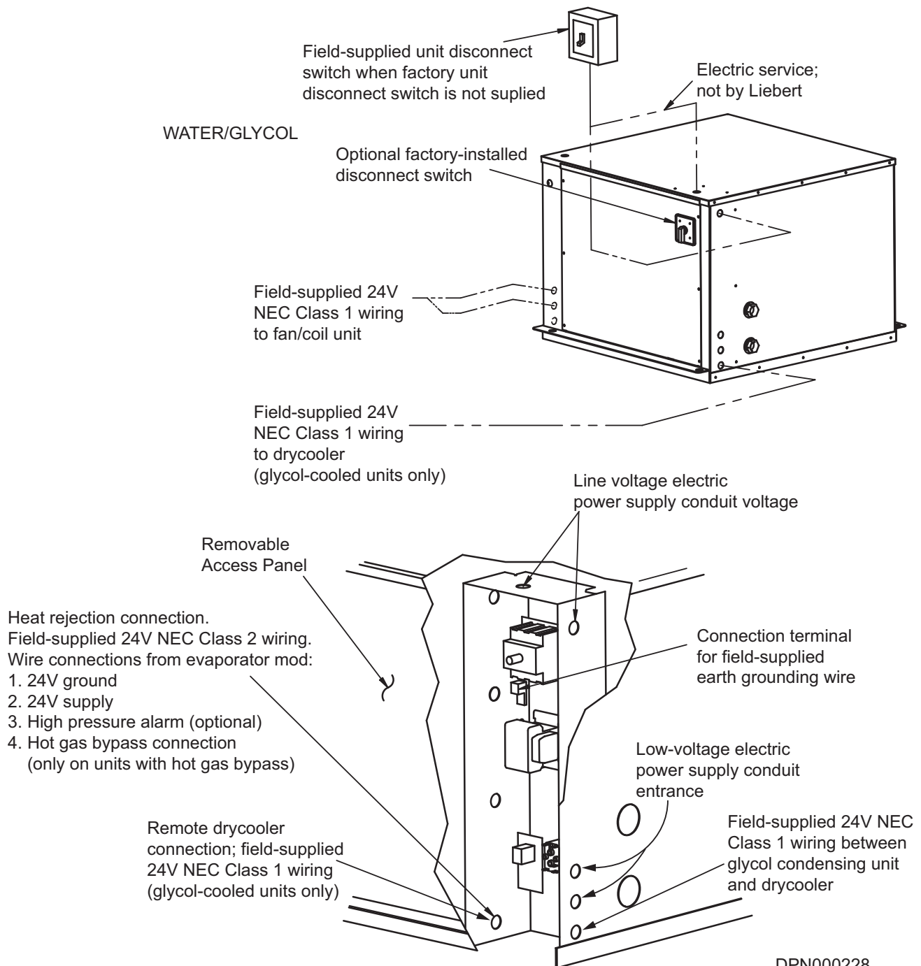
Figure 44 5-ton water/glycol-cooled condensing unit (con't.)
