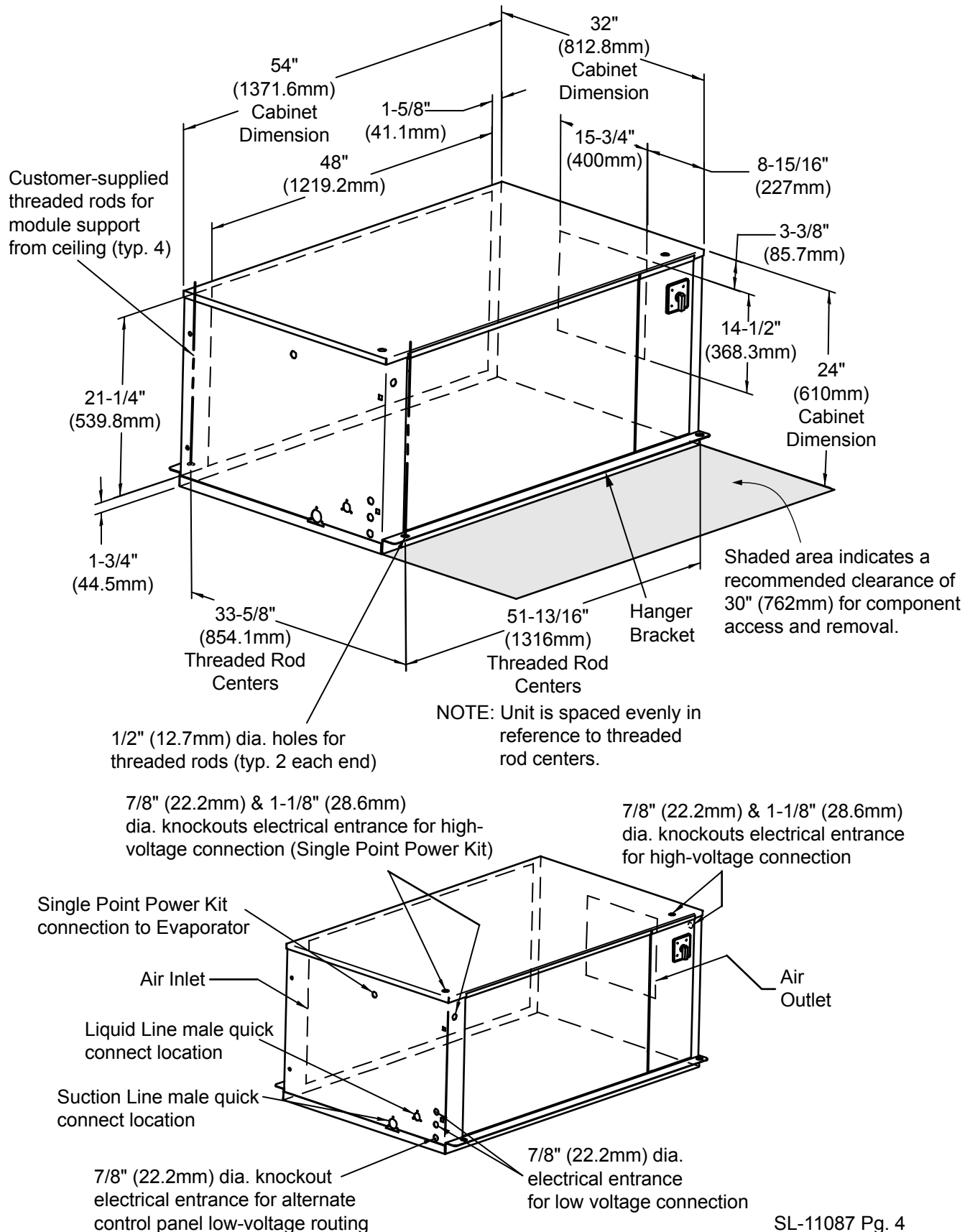
Figure 38 5-ton centrifugal air-cooled condensing unit dimensional data
