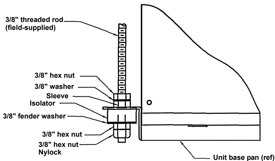
Figure 35 Detail of ceiling hanging bracket
