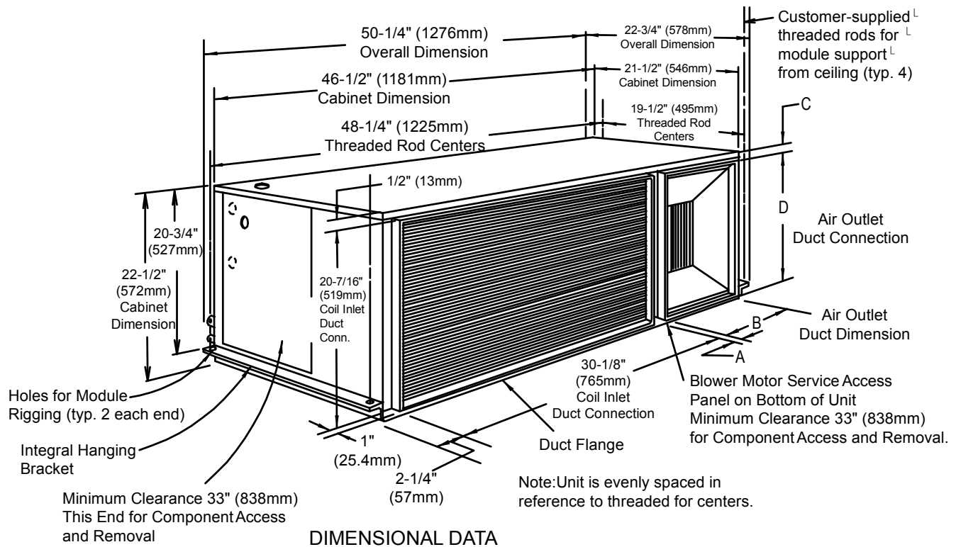
Figure 36 3-ton centrifugal air-cooled condensing unit dimensional data &amp; piping connections
