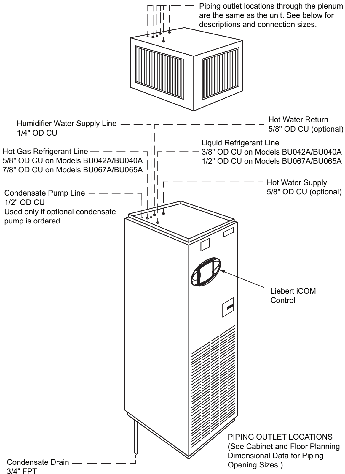
Figure 5 Piping connections for air-cooled units - Upflow models
